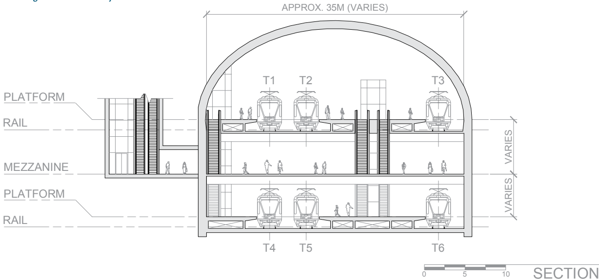
Underground Hub City 6-Track Station
