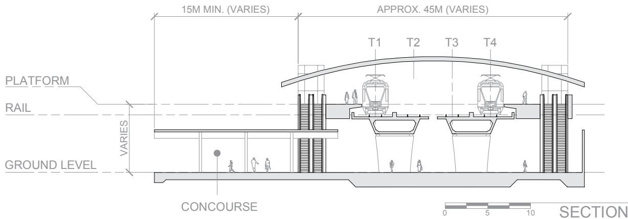
Elevated Suburban 4-Track Station
